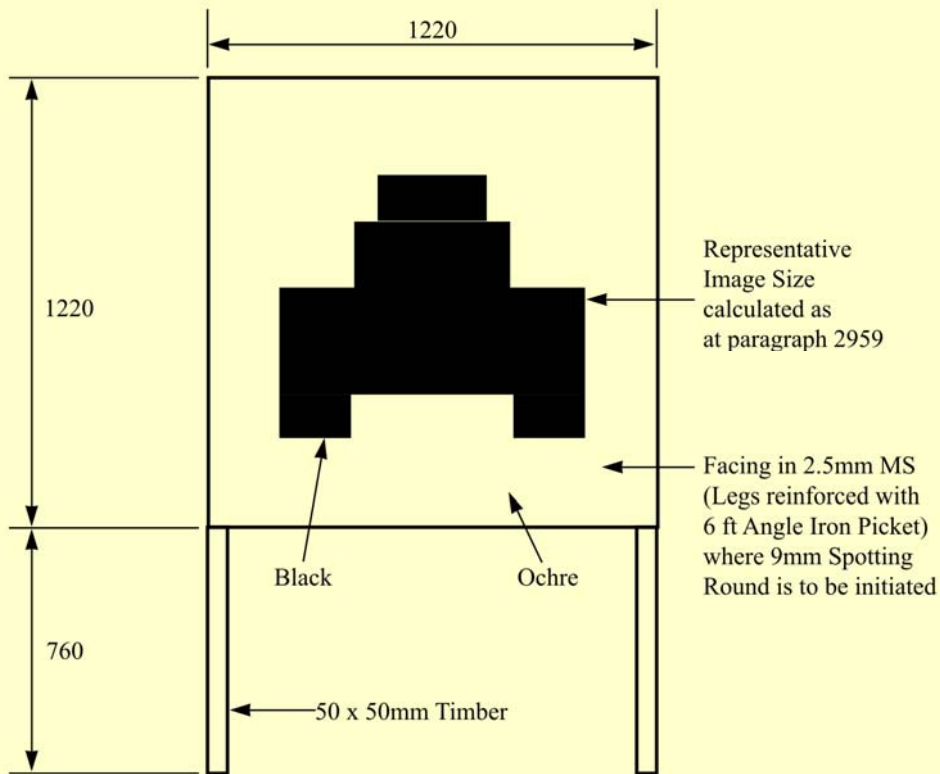
Head on Tank Target
