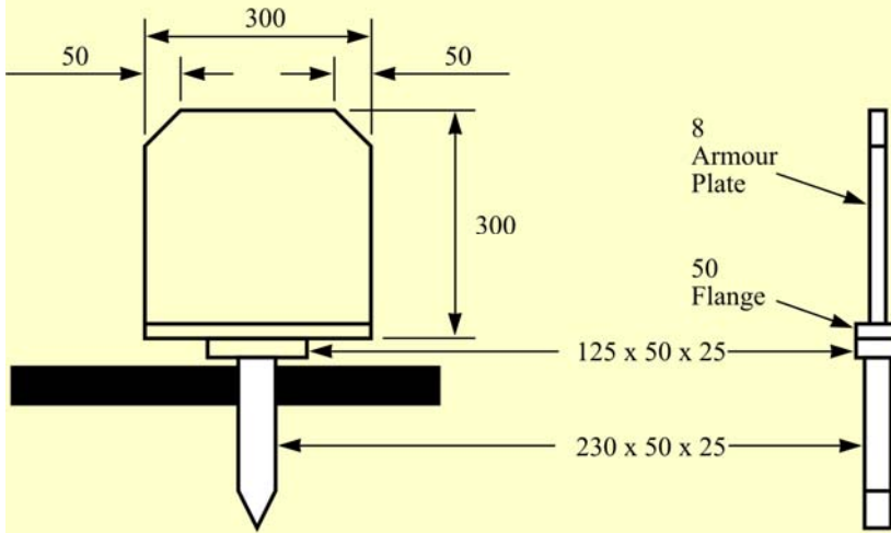
Falling Steel Plate (Catalogue of Royal Engineer Materiel Army Code 13535 Part No. 6920-99-439-0248)
